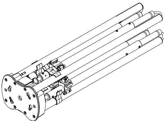
Aputure INFINIMAT Mounting Bracket 4×4
